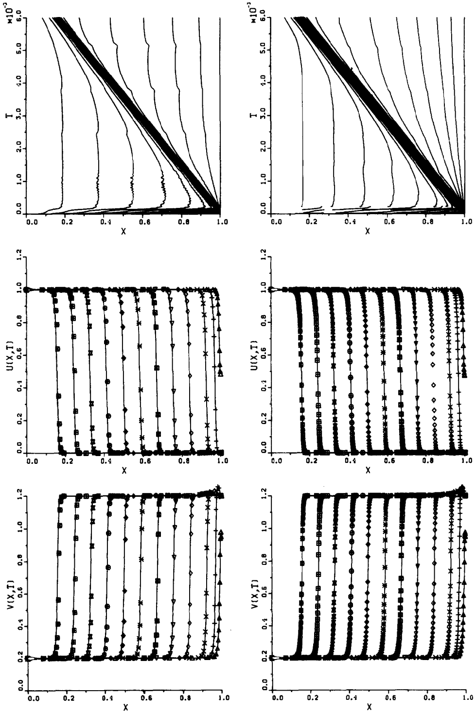
FIG. 5.3. Problem III. Grid trajectory and solutions at t = 0.15E-3, 0.3E-3, 0.6E-3 ( 0.6E-3 \sim 0.6E-2 ). Cases (i) (left) and (iv) (right).
